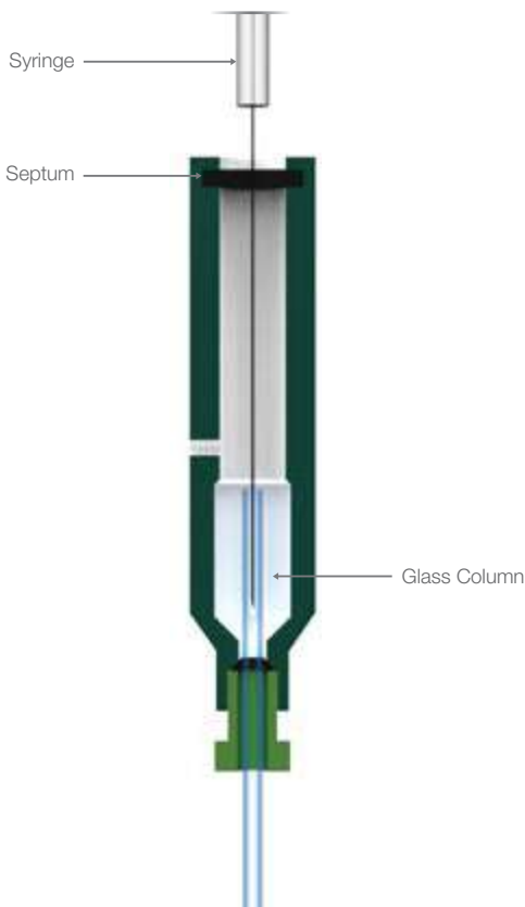
Syringes Figure 3. Illustration of an On-Column Injector
